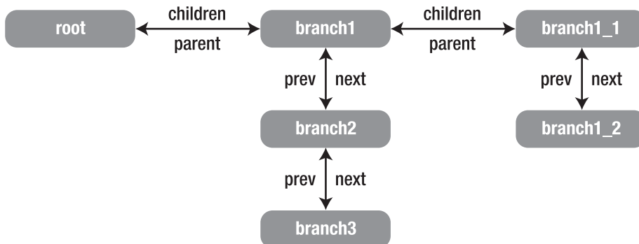
Figure 6-1. GNode relationships
